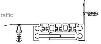
AR173-080 KÖŞE DETAYI AR173-080 CORNER DETAIL
