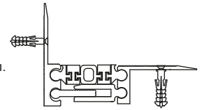
AR172-050 KÖŞE DETAYI AR172-050 CORNER DETAIL
