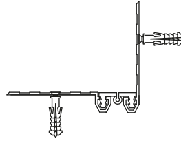
AR251-030 KÖŞE DETAYI AR251-030 CORNER DETAIL
