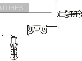
AR220-030 KÖŞE DETAYI AR220-030 CORNER DETAIL
