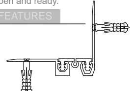
AR152-030 KÖŞE DETAYI AR152-030 CORNER DETAIL
