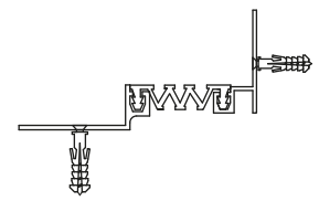
AR203-050 KÖŞE DETAYI AR203-050 CORNER DETAIL
