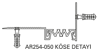
AR254-050 KÖŞE DETAYI AR254-050 CORNER DETAIL
