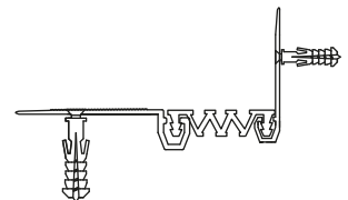
AR262-050 KÖŞE DETAYI AR262-050 CORNER DETAIL
