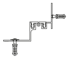
AR102-030 KÖŞE DETAYI AR102-030 CORNER DETAIL
