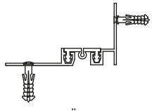
AR100-030 KÖŞE DETAYI AR100-030 CORNER DETAIL
