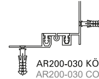
ALÇIPAN ASMA TAVAN ve BÖLME DUVAR DİLATASYON DETAYI DRYWALL CEILING PROFILE AND PARTITION WALL DILATATION DETAIL
