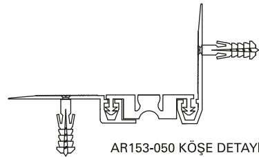
AR153-050 KÖŞE DETAYI AR153-050 CORNER DETAIL
