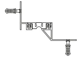
AR107-050 KÖŞE DETAYI AR107-050 CORNER DETAIL
