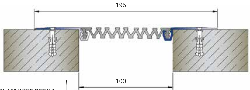
AR261-100 KÖŞE DETAYI AR261-100 CORNER DETAIL
