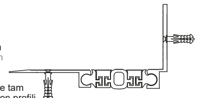
AR259-050 KÖŞE DETAYI AR259-050 CORNER DETAIL
