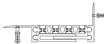
AR174-100 KÖŞE DETAYI AR174-100 CORNER DETAIL
