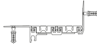
AR153-100 KÖŞE DETAYI AR153-100 CORNER DETAIL
