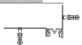
AR255-030 KÖŞE DETAYI AR255-030 CORNER DETAIL
