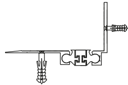
AR258-030 KÖŞE DETAYI AR258-030 CORNER DETAIL
