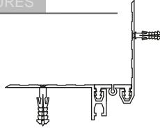
AR150-030 KÖŞE DETAYI AR150-030 CORNER DETAIL
