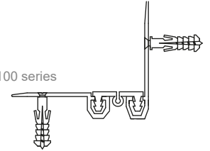
AR260-030 KÖŞE DETAYI AR260-030 CORNER DETAIL
