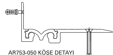
AR753-050 KÖŞE DETAYI AR73-050 CORNER DETAIL
