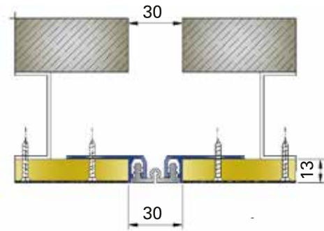
ALÇIPAN ASMA TAVAN ve BÖLME DUVAR DİLATASYON DETAYI DRYWALL CEILING PROFILE AND PARTITION WALL DILATATION DETAIL
