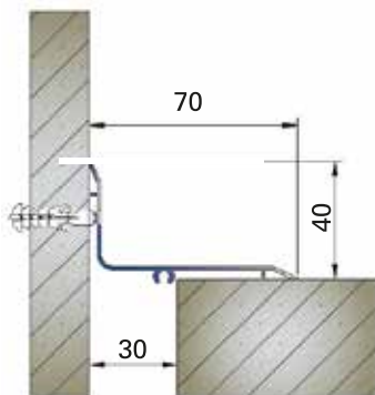
AR4070K (Köşe Kapak) AR4070K (Corner Cover)
