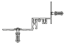
AR101-030 KÖŞE DETAYI AR101-030 CORNER DETAIL
