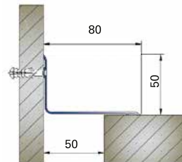
AR5080K (Köşe Kapak) AR5080K (Corner Cover)
