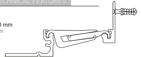
AR712-080 KÖŞE DETAYI AR712-080 CORNER DETAIL
