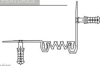
AR261-050 KÖŞE DETAYI AR261-050 CORNER DETAIL
