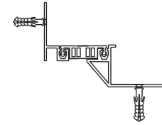
AR107-052 KÖŞE DETAYI AR107-052 CORNER DETAIL
