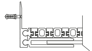
AR174-150 KÖŞE DETAYI AR174-150 CORNER DETAIL
