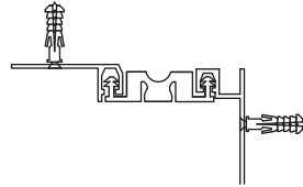
AR202-051 KÖŞE DETAYI AR202-051 CORNER DETAIL
