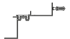
AR221-030 KÖŞE DETAYI AR221-030 CORNER DETAIL
