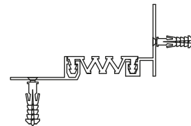
AR202-050 KÖŞE DETAYI AR202-050 CORNER DETAIL
