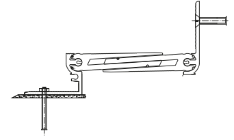
AR823-150 KÖŞE DETAYI AR823-150 CORNER DETAIL
