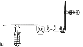
AR262-051 KÖŞE DETAYI AR262-051 CORNER DETAIL
