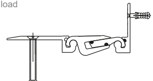
AR763-080 KÖŞE DETAYI AR763-080 CORNER DETAIL
