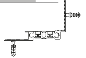
AR209-050 KÖŞE DETAYI AR209-050 CORNER DETAIL
