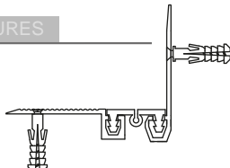
AR154-030 KÖŞE DETAYI AR154-030 CORNER DETAIL
