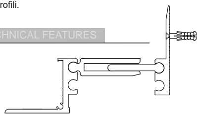
AR309-080 KÖŞE DETAYI AR309-080 CORNER DETAIL
