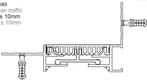
AR109-081 KÖŞE DETAYI AR109-081 CORNER DETAIL
