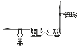
AR154-050 KÖŞE DETAYI AR154-050 CORNER DETAIL
